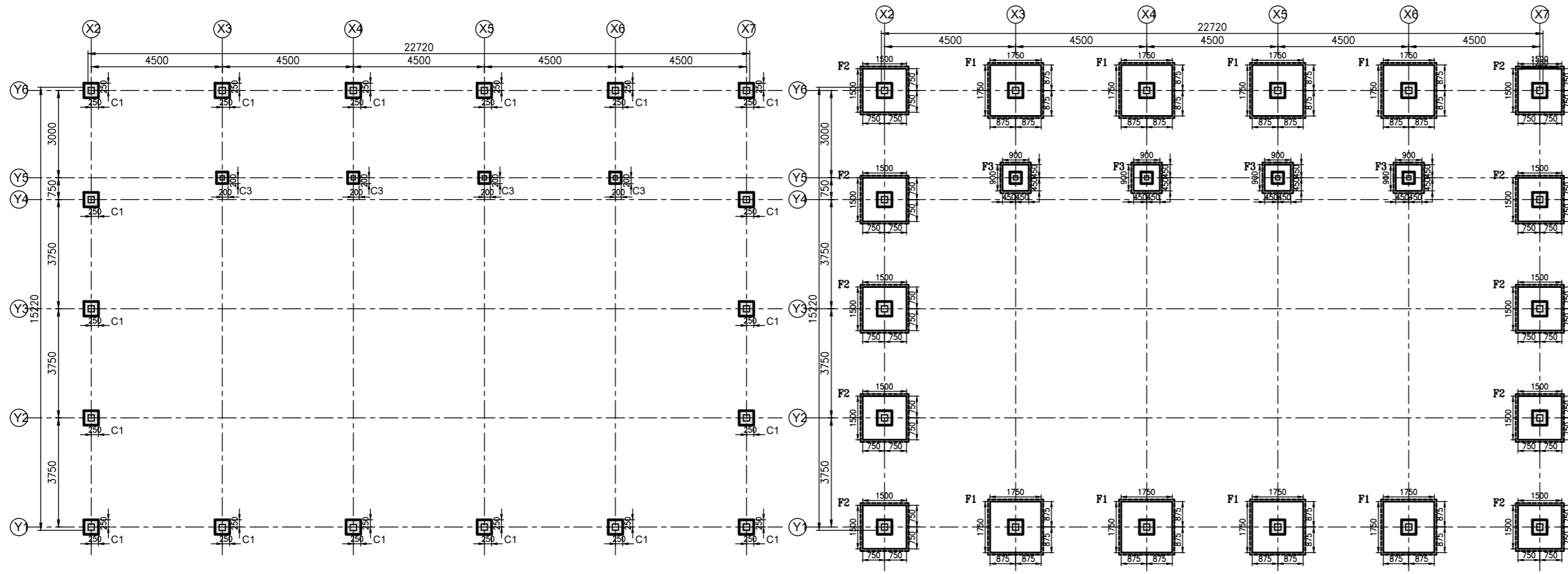
COLUMN LAYOUT
