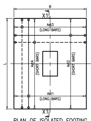
PLAN OF ISOLATED FOOTING
